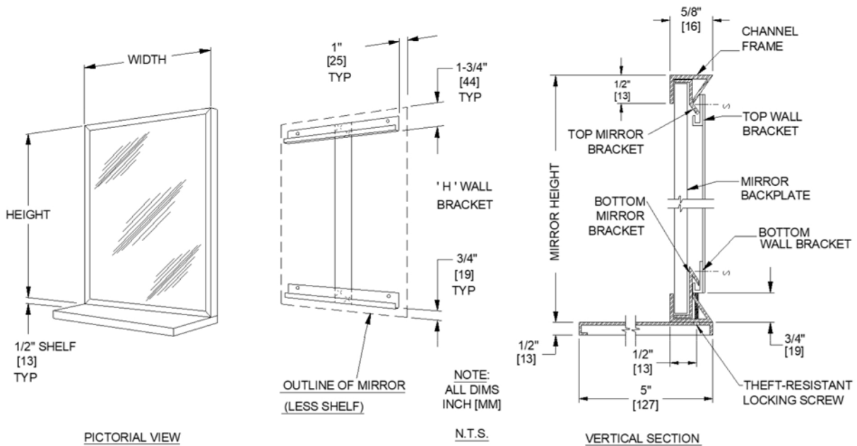
PICTORIAL VIEW
